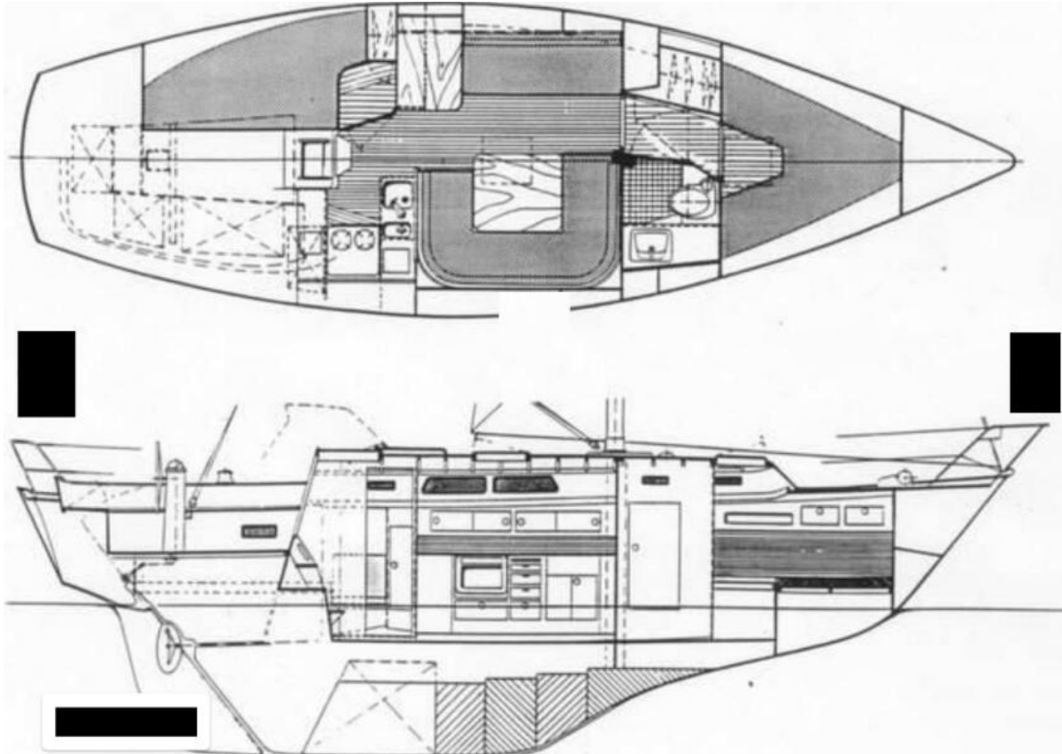
Arrangement Plan
