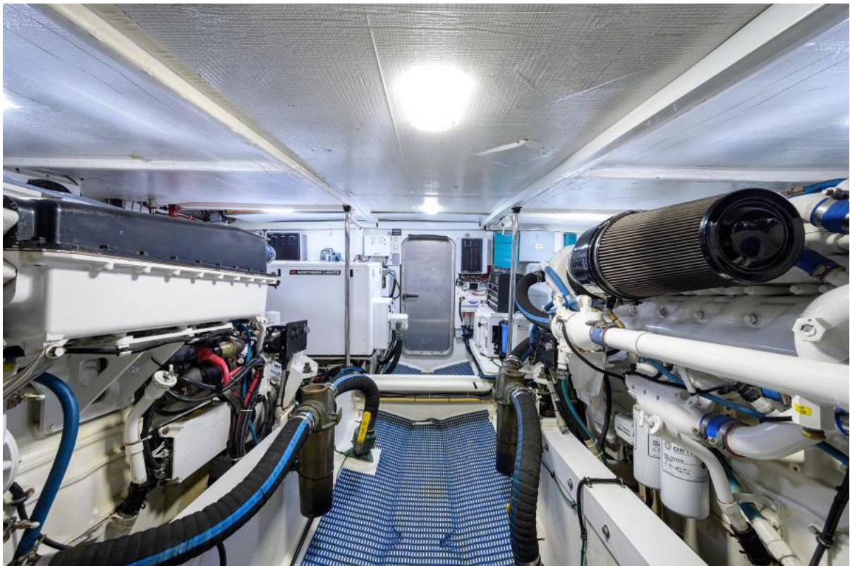
Pacific Mariner 65 Last Call - Engine Room 2009 Pacific Mariner 65 - Last Call
