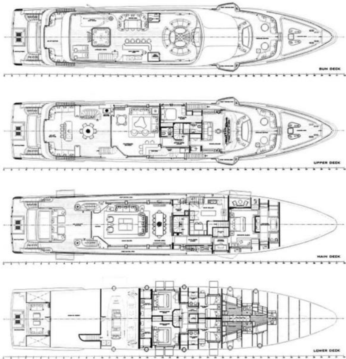
General Arrangement
