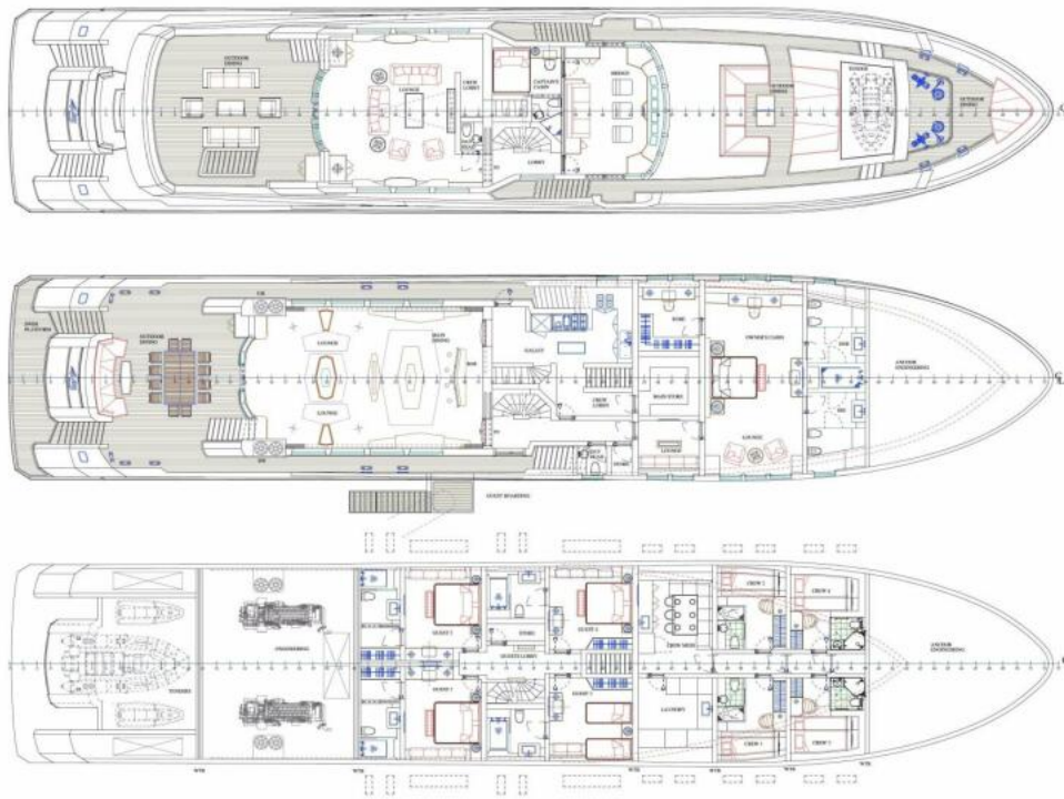
General Arrangement
