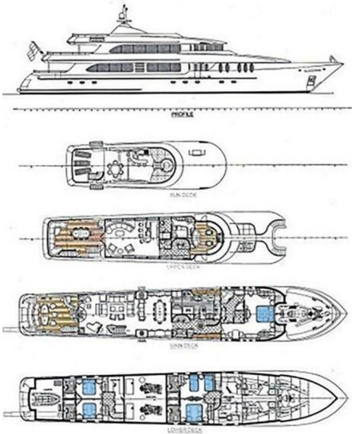
General Arrangement
