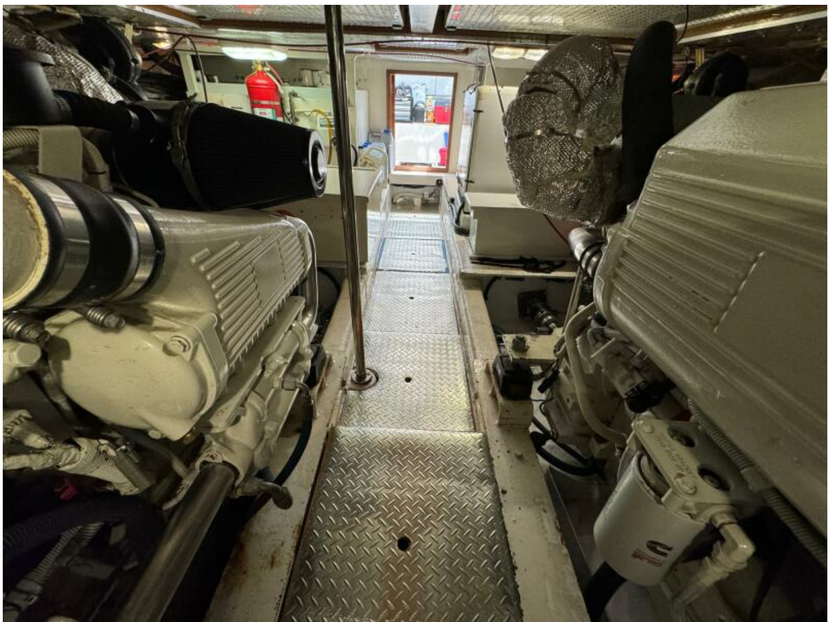
79 2007 52 Jefferson Pilothouse Engine Room
