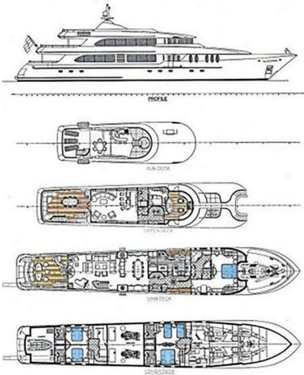
General Arrangement
