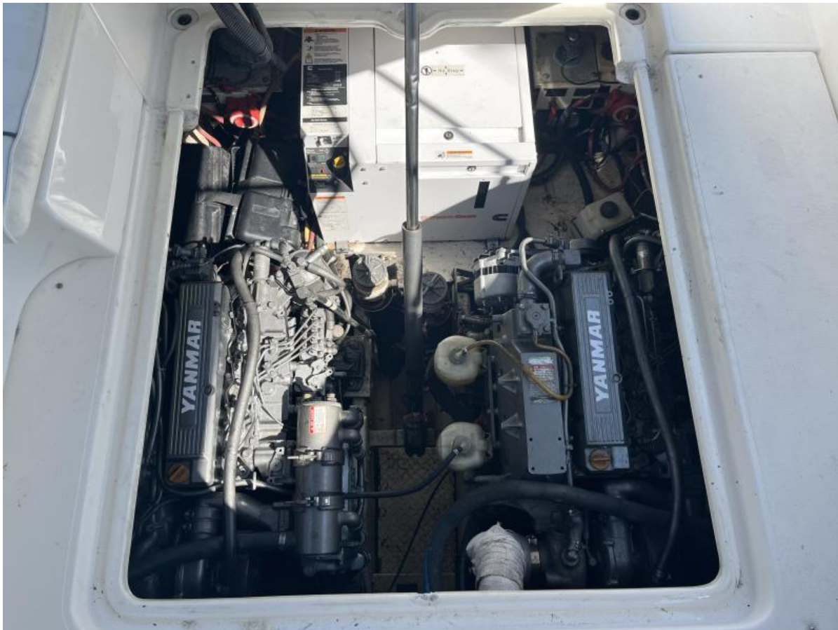
2005 Cruisers 340 Express Engines
