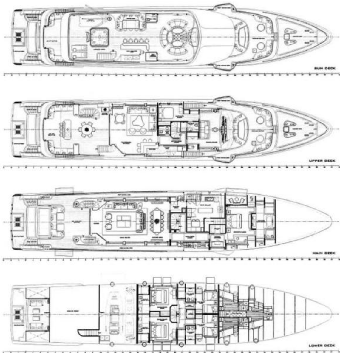
General Arrangement
