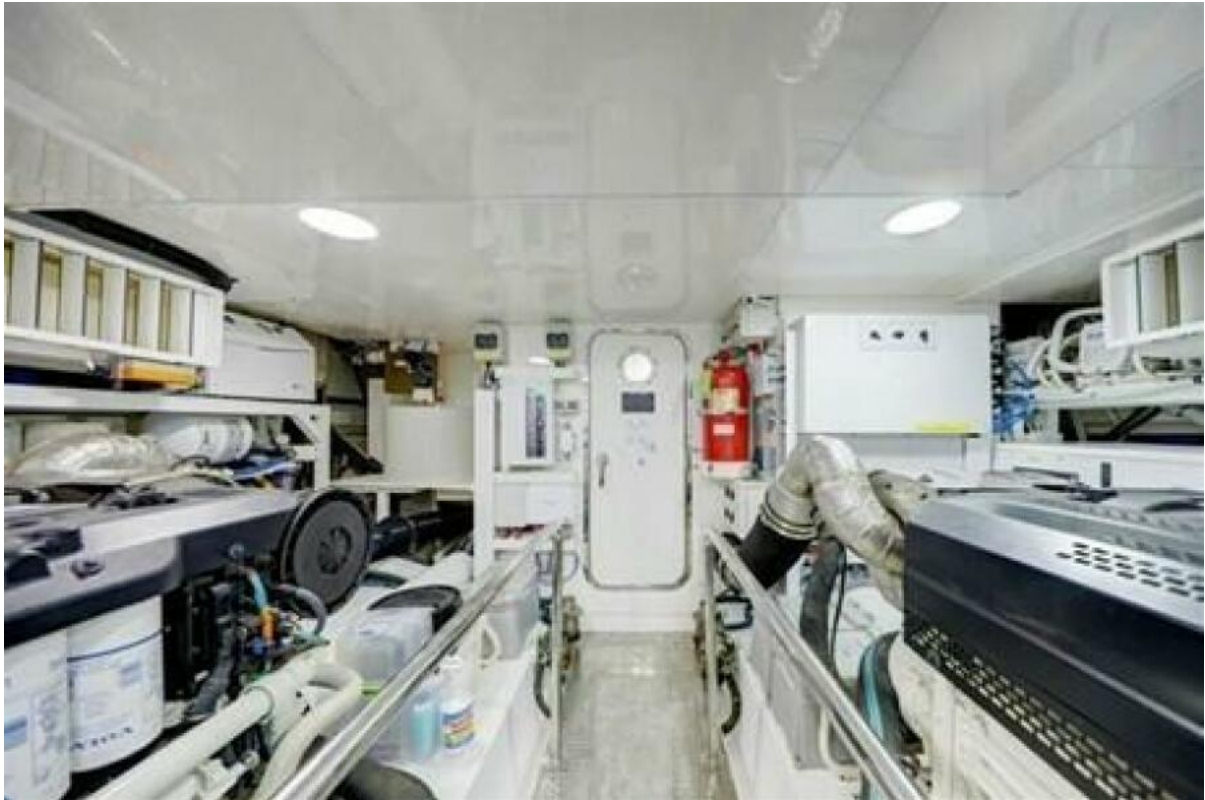
Engine Room
