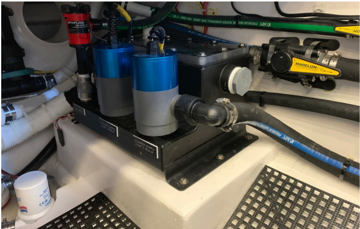
Valhalla 41 - Engine Room 2022 Valhalla Boatworks V41
