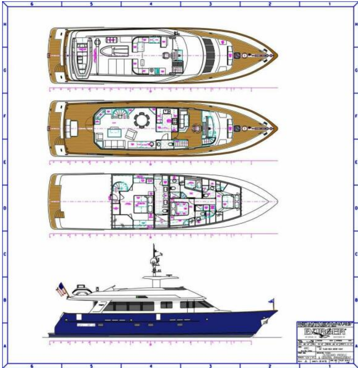
Layout
