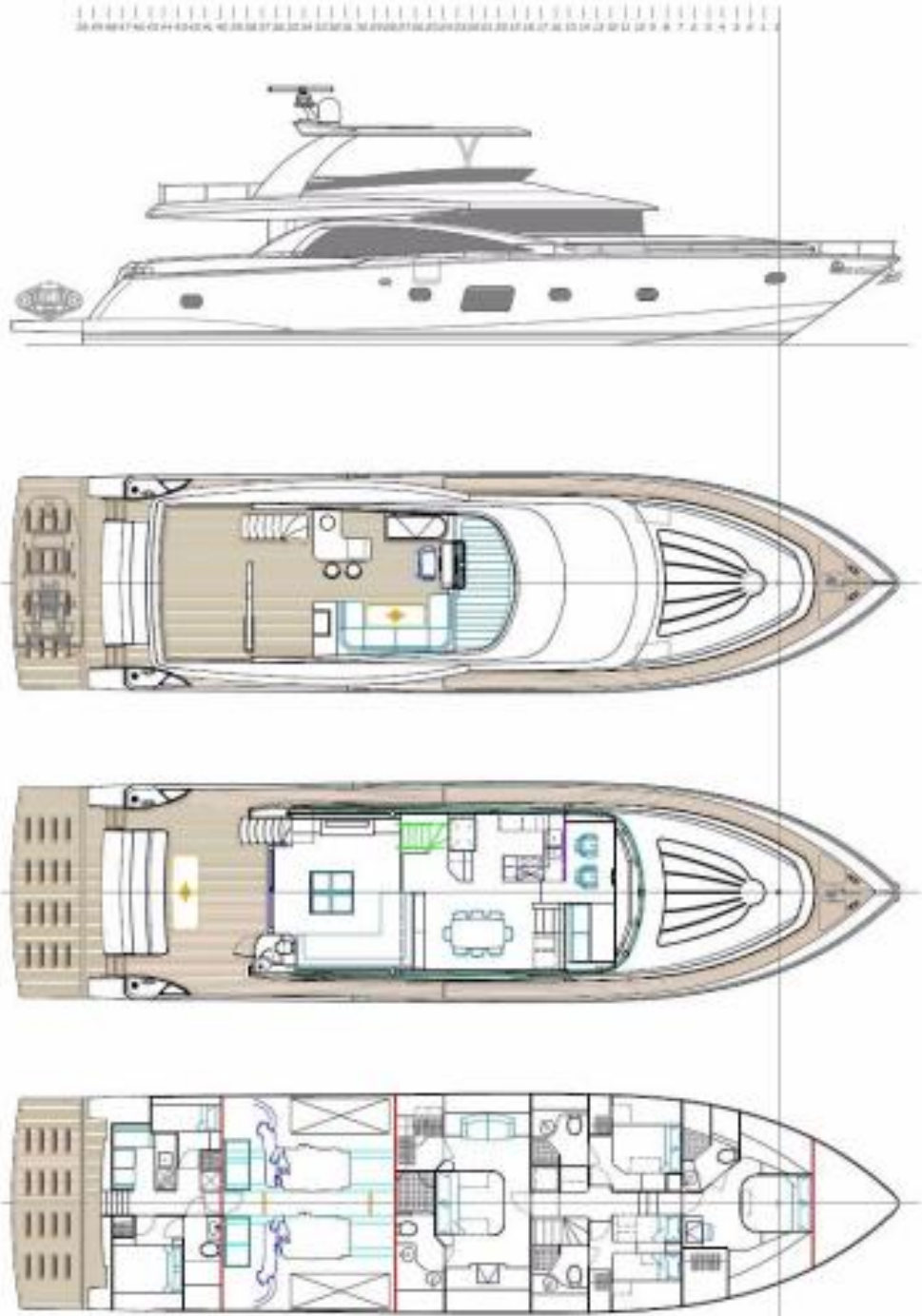
JOHNSON YACHTS CO., LTD 83' OPEN FLYBRIDGE GENERAL LAYOUT (HYDRAULIC PLATFORM)
