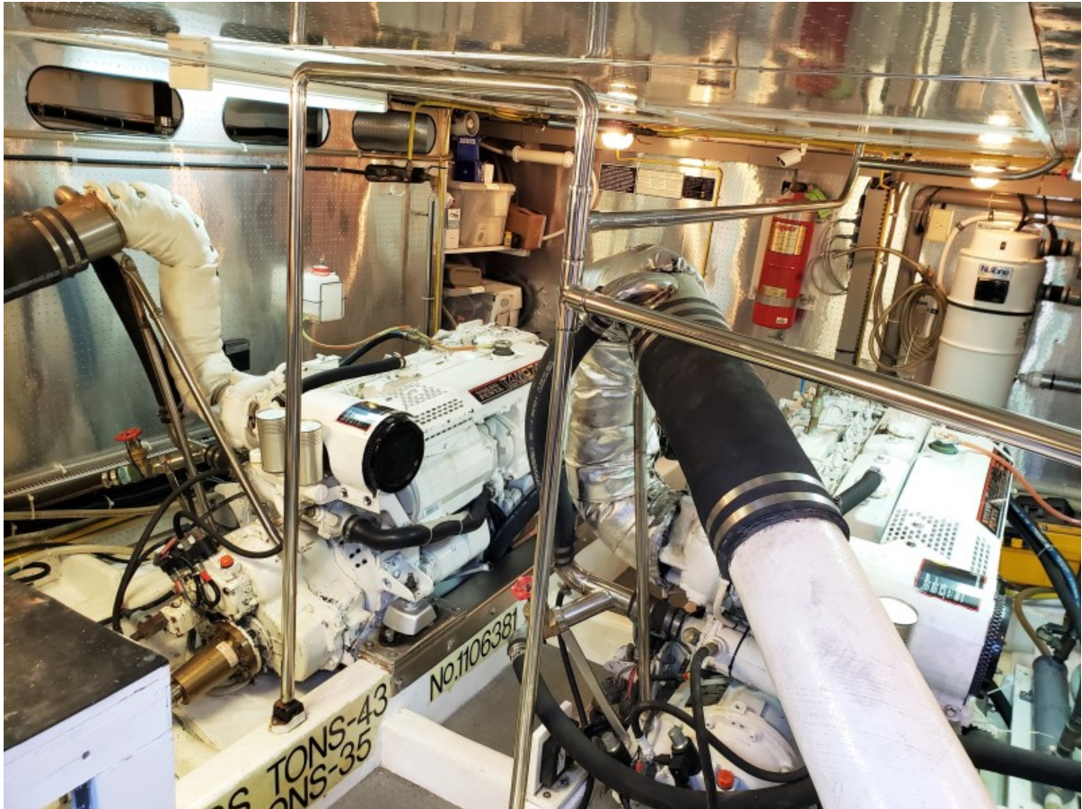
Eng room 2
