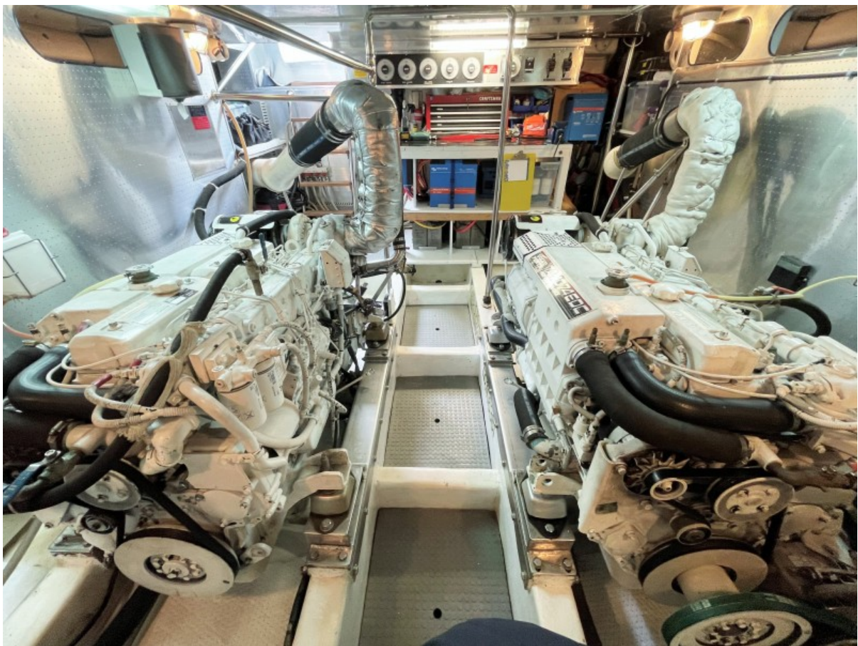
Eng room 3
