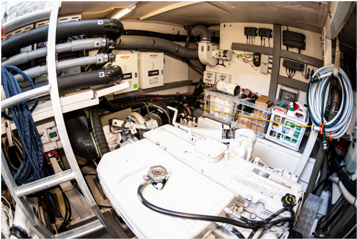
2014 58 Prestige 550 Sweet Annie Engine Room Starboard
