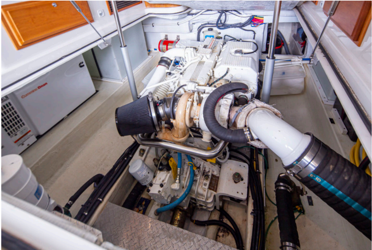
Engine Area
